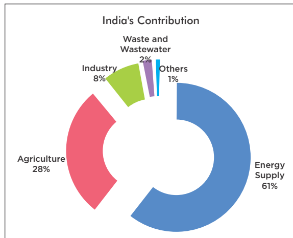
Greenhouse Gases caused due to economic activities. 3
