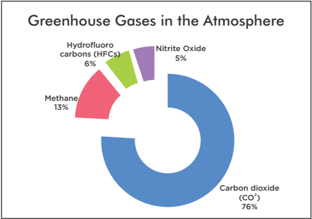
These are the main greenhouse gases that are present in our atmosphere. Carbon dioxide (CO 2 ) is the most significant and produced abundantly. 1
